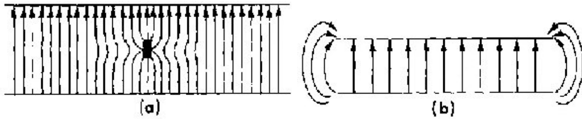
Figure 3.10 (a) E -field lines when a small metallic object is placed between the plates. (b) E -field lines between parallel conducting plates of finite size.
