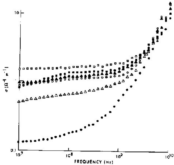
Figure 4.28. The conductivity of ocular tissues at 37°C (Gabriel et al., 1983). Key: ■ retina, ○ iris, ▲ choroid, □ cornea, Δ lens cortex, and ● lens nucleus.
