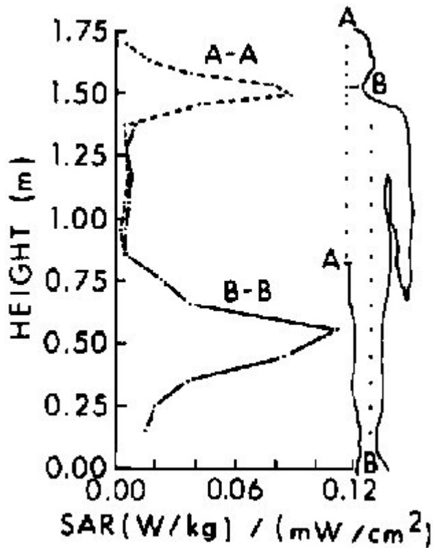
Figure 8.47. SAR distribution along an average man-model height for two cross sections; 1\text{-mW/cm}^2 incident-power density on the surface of the model, frequency 350 MHz E\parallel L , K back to front (Krazewski et al., 1984) (© 1984 IEEE).
