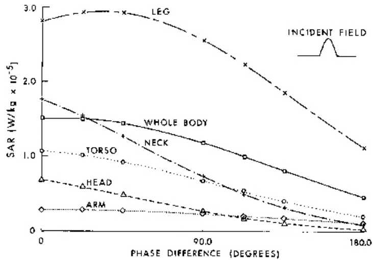
Figure 6.47. Whole- and part-body SAR at 77 MHz in the block model of man as a function of an assumed linear antisymmetric phase variation in the incident E_z ; E_z|_{max} = 1 V/m. Calculated by Chatterjee et al. (1980a, 1980b, 1980c).
