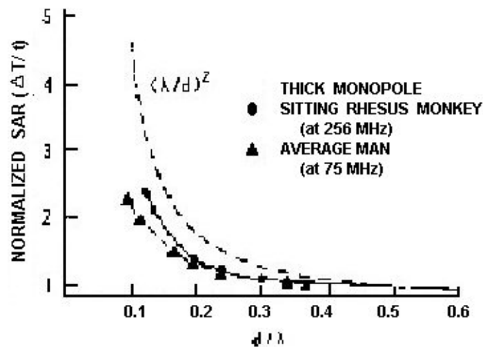
Figure 8.19. Measured relative SARs in scaled saline spheroidal models of man. To emphasize the differences in the absorption characteristics, the values are normalized with respect to their far-field value at d/\lambda = 0.5 . \Delta T is the temperature rise in the saline solution after exposure for time t (Iskander et al., 1981).
