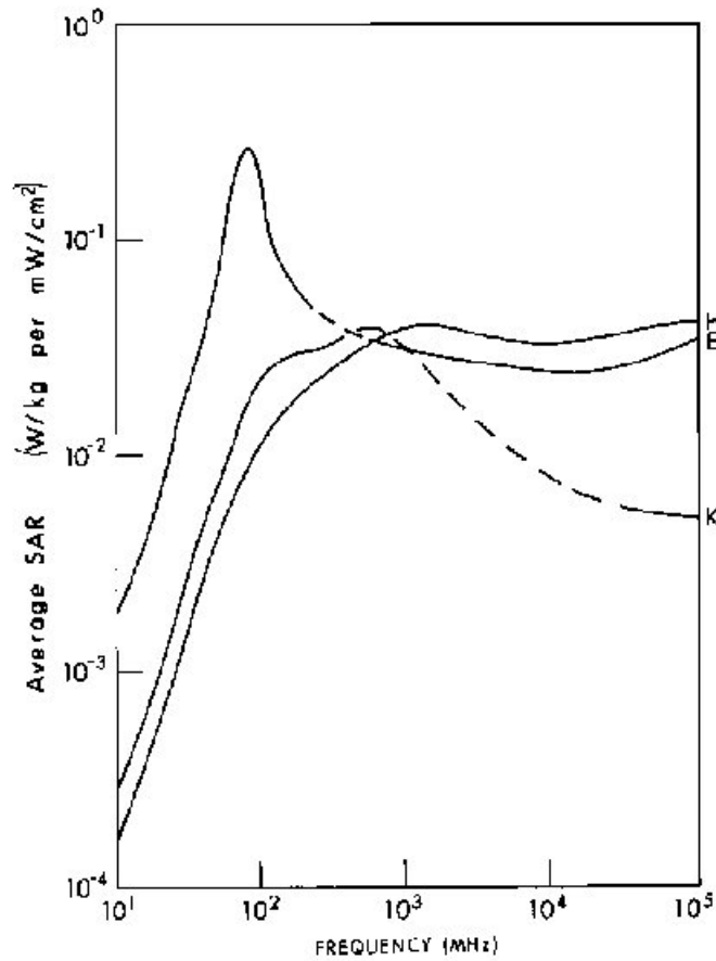
Figure 3.39. Calculated whole-body average SAR frequency for model of an average man for three standard polarizations. The incident-power density is 1 \text{ mW/cm}^2 .
