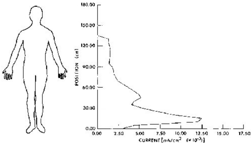
Figure 9.16. Calculated current distribution as a function of position in man with hand contacting a large object and with feet grounded. A 1-mA current is assumed to floating through the arm, thorax, and legs of the subject to the ground, F=60 Hz (Guy and Chou, 1982).
