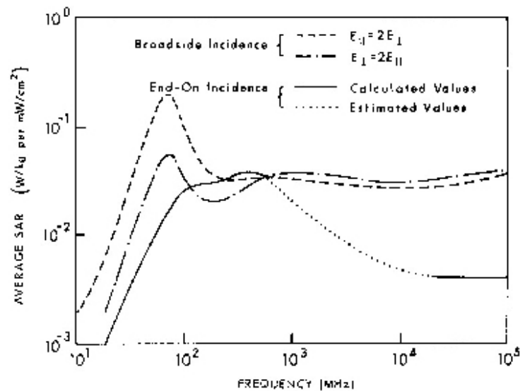
Figure 6.28. Calculated planewave average SAR in a prolate spheroidal model of an average man irradiated by an elliptically polarized wave, for two orientations; a = 0.875 m, b = 0.138 m, V = 0.07 m 3 .
