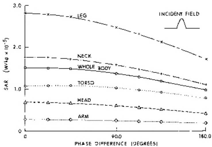
Figure 6.48. Whole- and part-body SAR at 77 MHz in the block model of man as a function of an assumed linear symmetric phase variation in the incident E_z ; E_z|_{max} = 1 V/m. Calculated by Chatterjee et al. (1980a, 1980b, 1980c).
