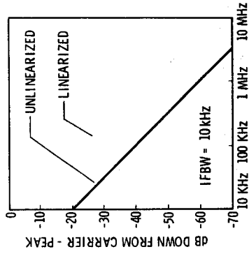
Fig. 11. Noise characteristics of a 4-8 GHz unlinearized and linearized VCO.
